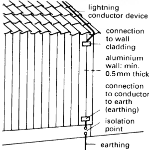
③ The main components of a lightning protection system
